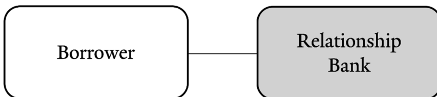
FIGURE 1. RELATIONSHIP LENDING
